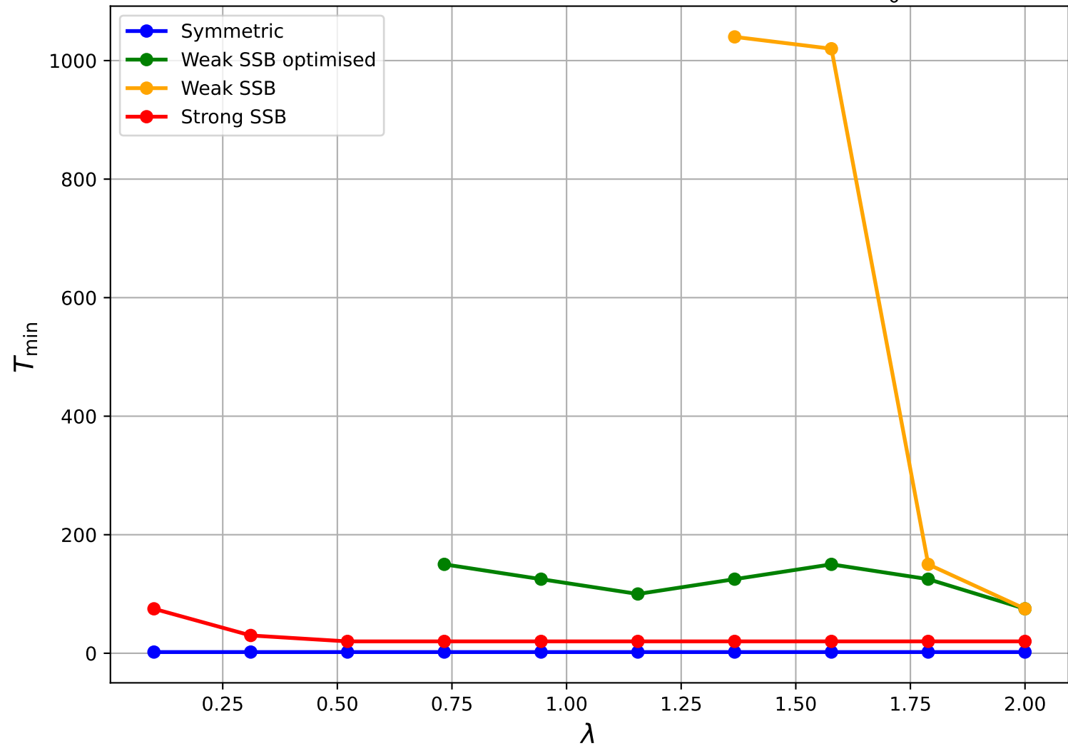
Minimum Adiabatic Time T_{\min} for Fidelity \geq 0.99 , m_0^2 = 1.0
